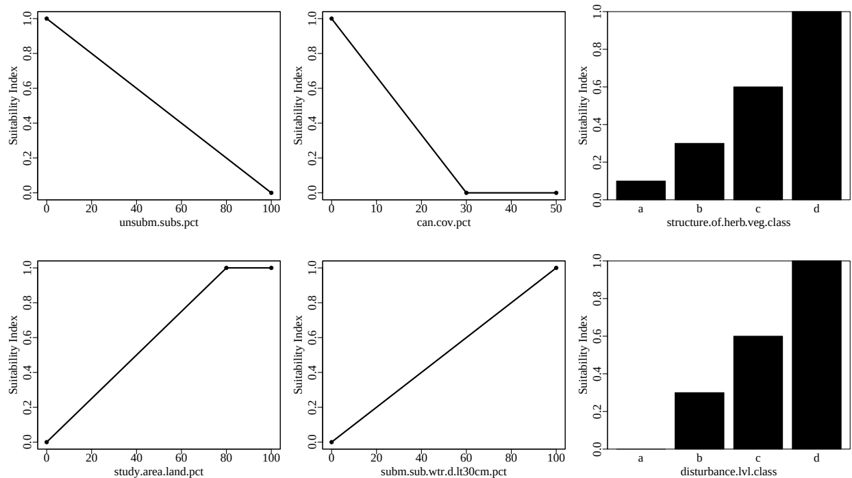
Figure 1. Suitability index graphs for variables included in the mottledduckNesting model in ecorest .
